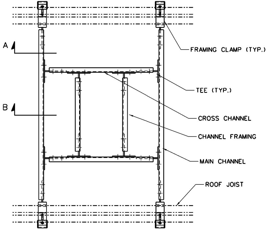
BASIC FRAME WITH ADDITIONAL CHANNEL SUPPORTS
